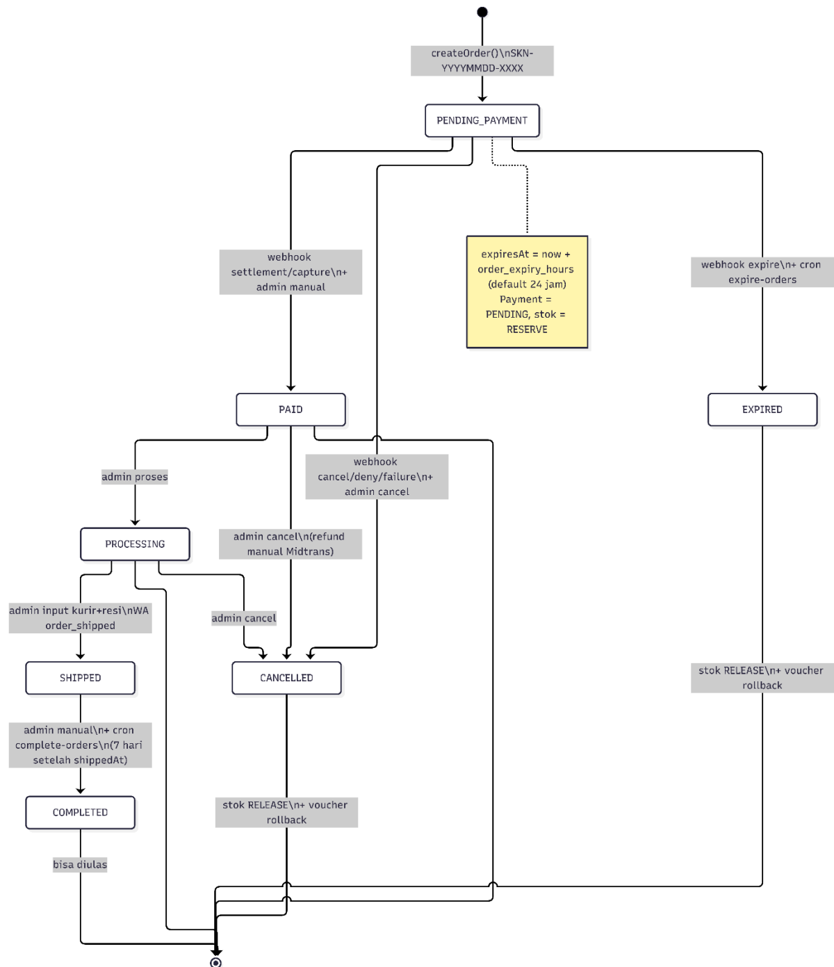
Gambar 7.5 State Diagram Status Pesanan
