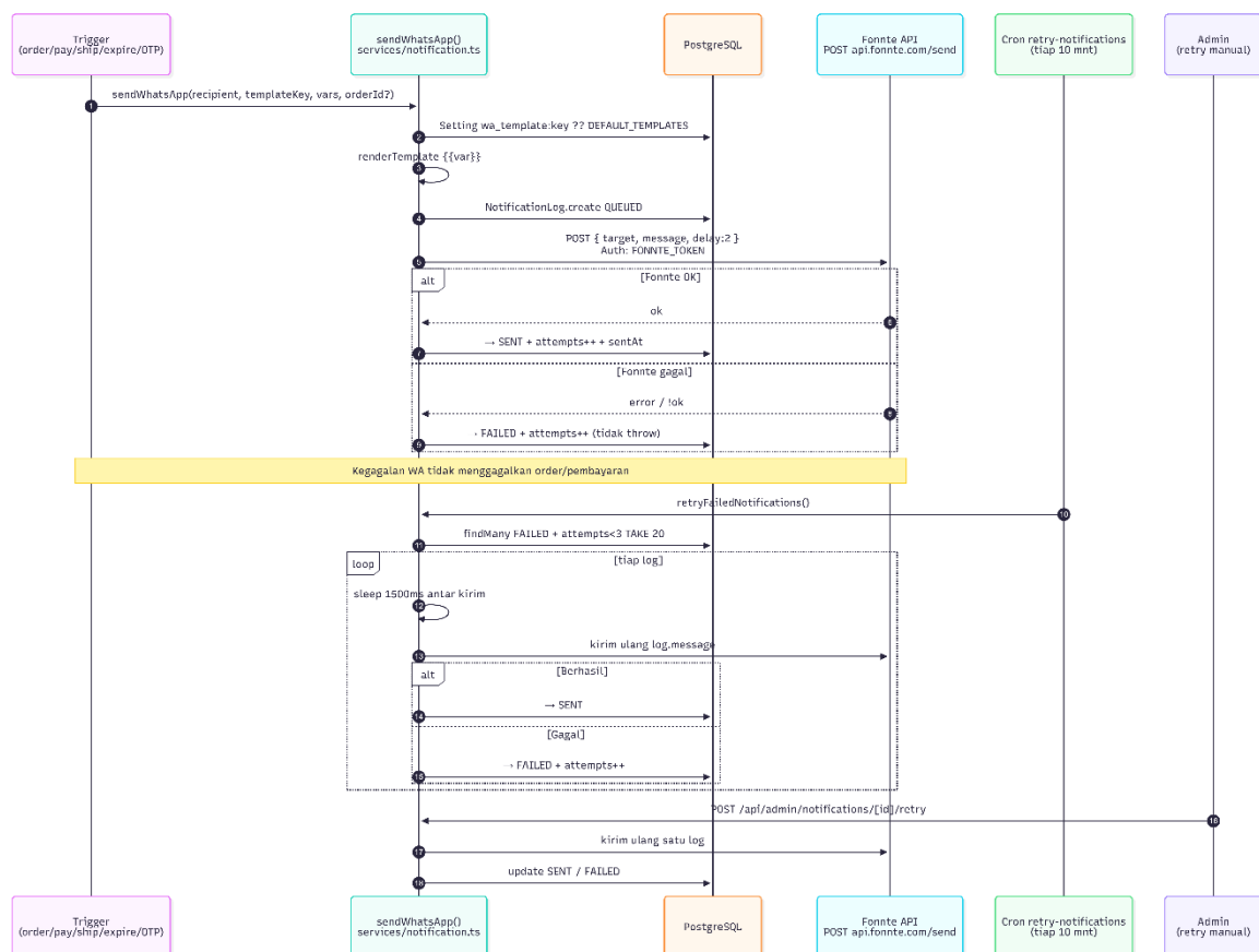
Gambar 11.1 Sequence Diagram Pengiriman Notifikasi & Retry
