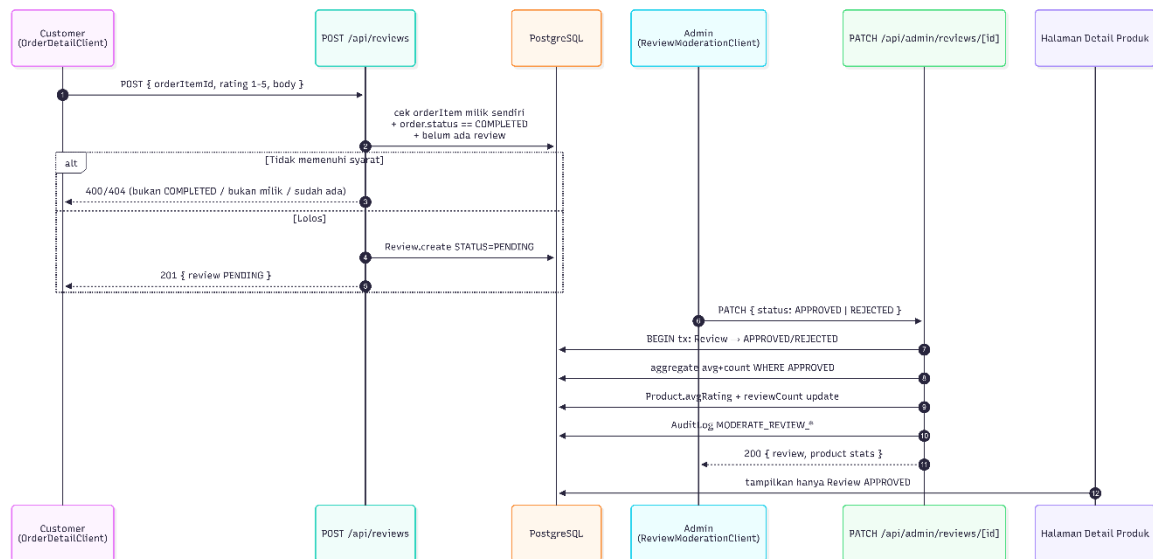
Gambar 7.7 Sequence Diagram Ulasan &amp; Moderasi
