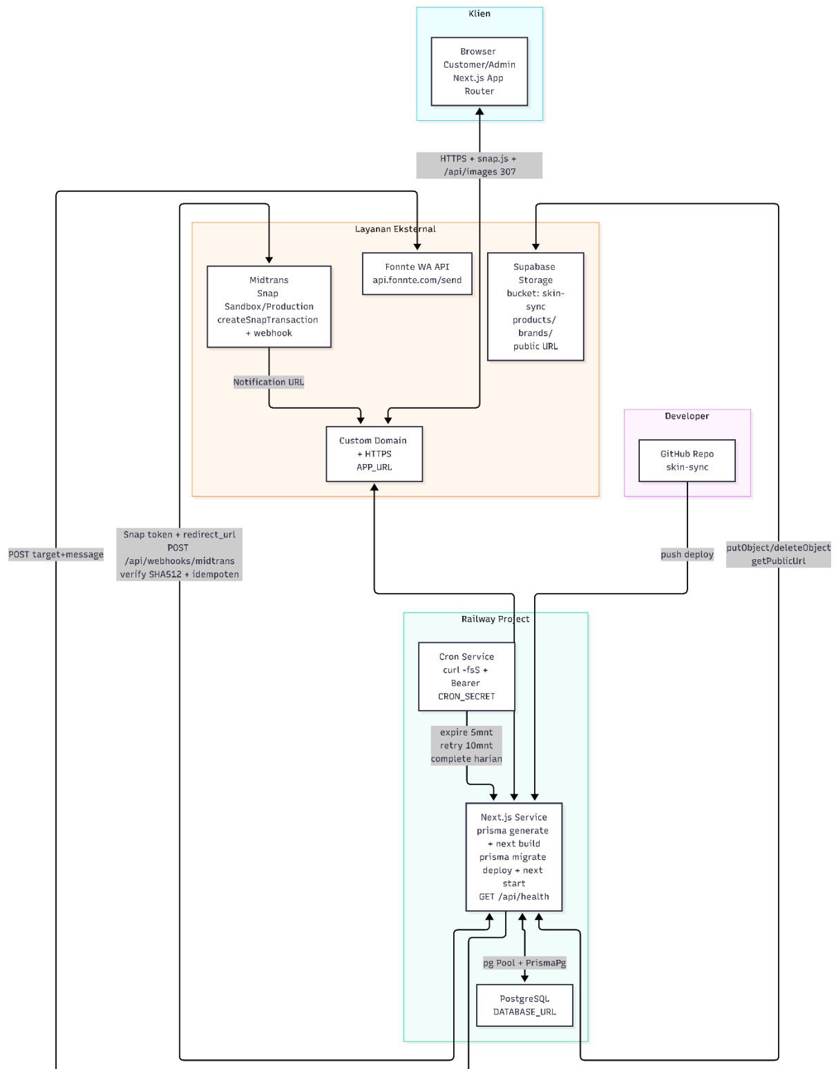
Gambar 14.1 Diagram Deployment
