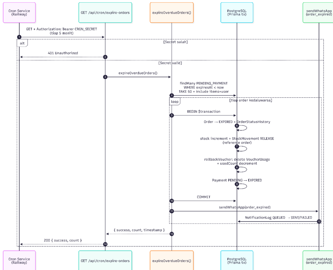
Gambar 7.6 Sequence Diagram Cron Kedaluwarsa Pesanan
